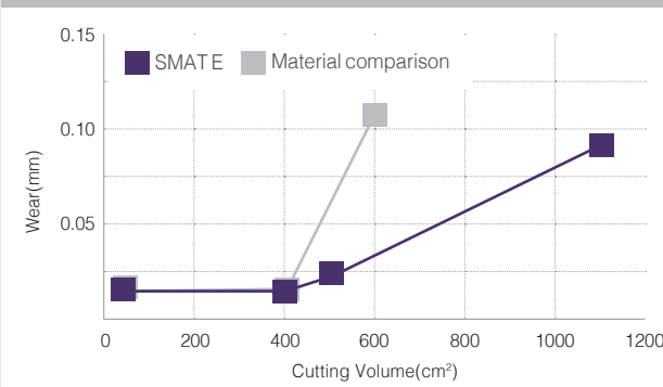
End-Mill((WC material, diameter of 16Φ)
