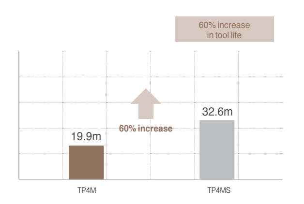
Gun Drill Machining [Gun Drill Machining Length]
