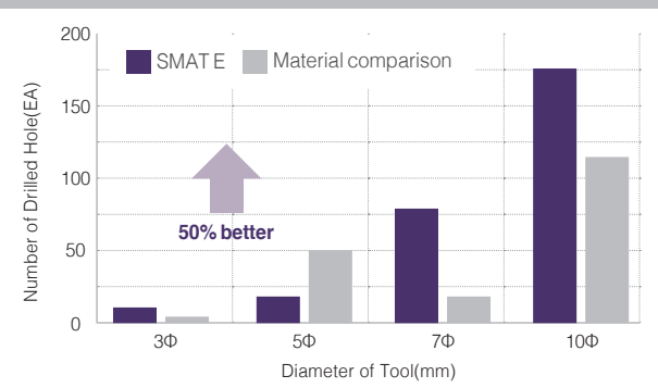
Drill(HSS material)
