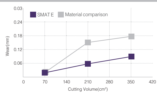
End-Mill(HSS material, diameter of 16Φ)
