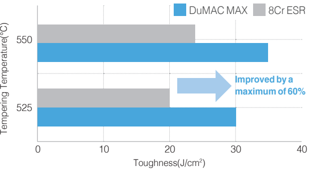
Impact Toughness
