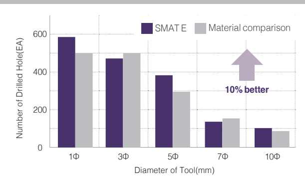
Drill(WC material)
