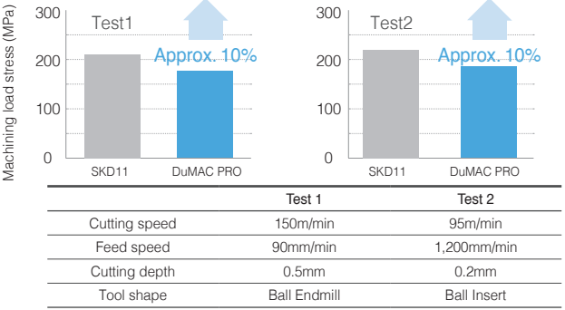
Machinability
