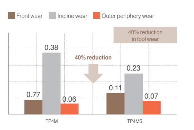
End Mill Machining [Comparison of Tool Wear]
